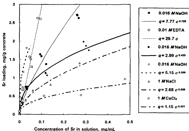
FIGURE 3. Results of strontium equilibration tests.
