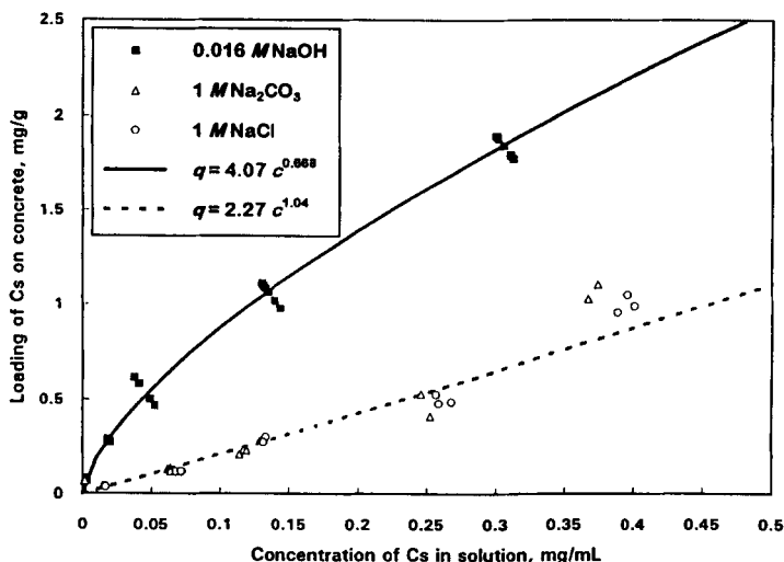
FIGURE 2. Results of cesium equilibration tests.
