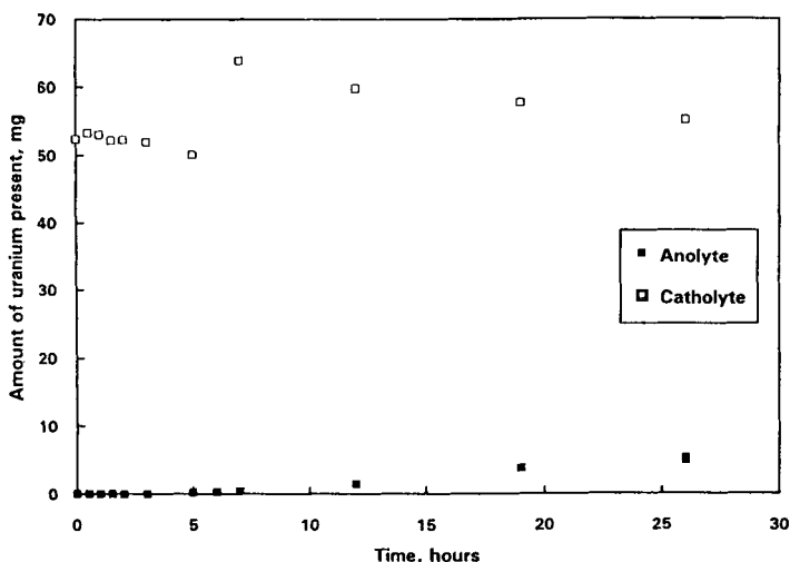
FIGURE 8. Variation of uranium in anolyte and catholyte during dynamic test using 1 M carbonate solutions as initial anolyte and catholyte.
