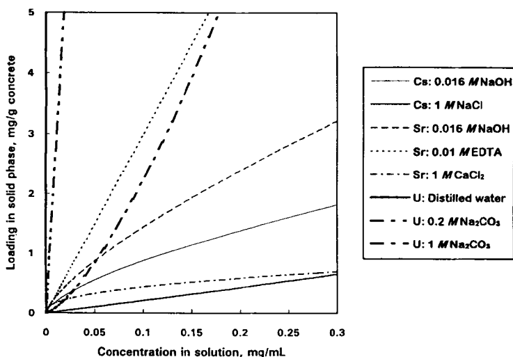
FIGURE 5. Summary of equilibration test results.
