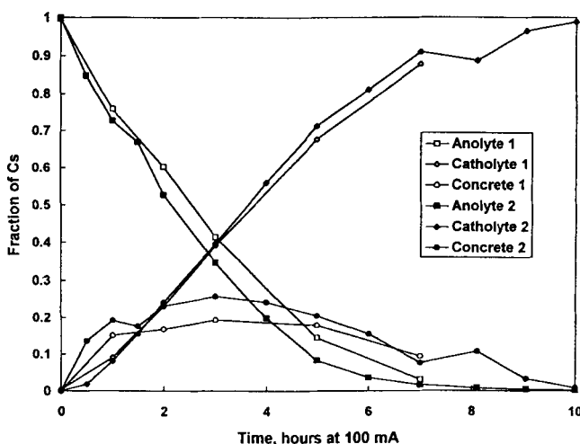
FIGURE 6. Results of cesium dynamic tests, indicating the variation of the distribution of cesium between the anolyte, catholyte, and concrete.
