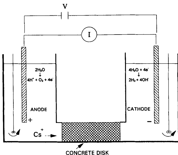
FIGURE 1. Schematic of dynamic electrokinetic experiment.
