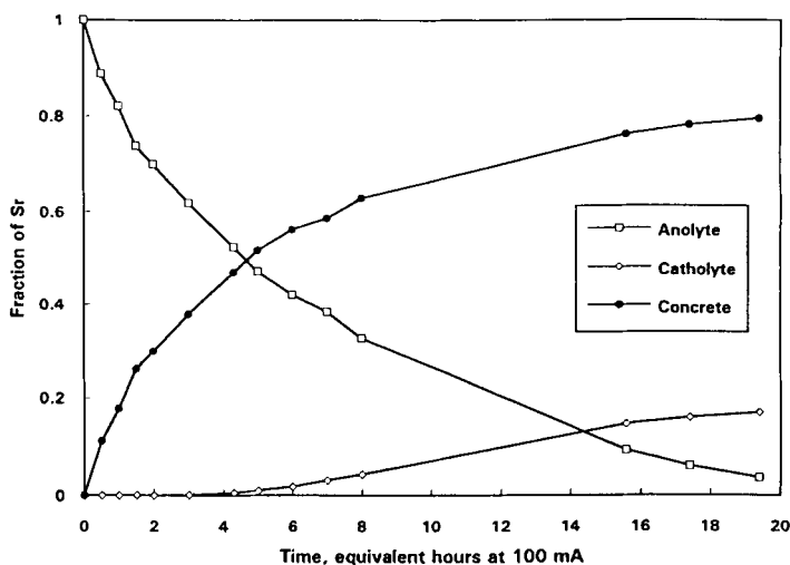
FIGURE 7. Results of strontium dynamic test, indicating the variation of the distribution of strontium between the anolyte, catholyte, and concrete.
