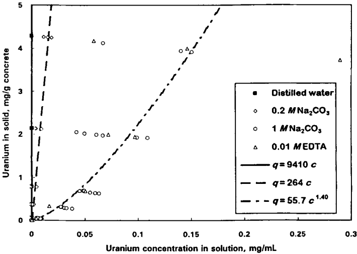
FIGURE 4. Results of uranium equilibration tests.
